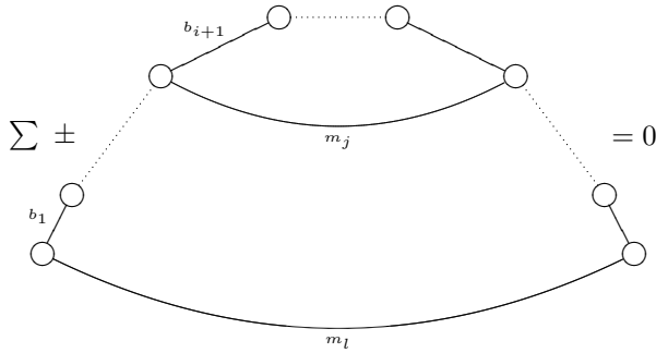
FIGURE 4.6: A_\infty -identities.
