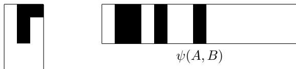
FIGURE 8.1: Kalman code and bar code.
