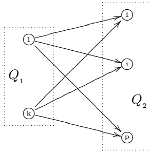
FIGURE 7.2: Free product of quivers.
