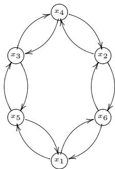
FIGURE 7.3: The local quiver.
