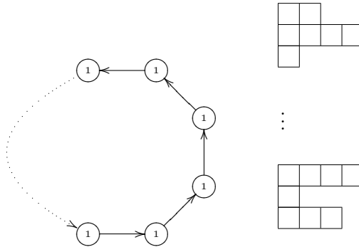
FIGURE 6.9: Local quiver settings for curve orders.
