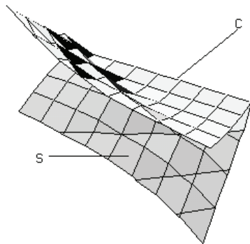
FIGURE 1.3: Representation strata for 3 \times 3 matrices.
