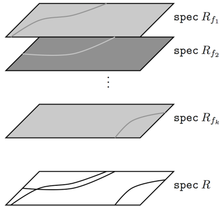
FIGURE I.2: A Zariski cover of X = \text{spec } R .
