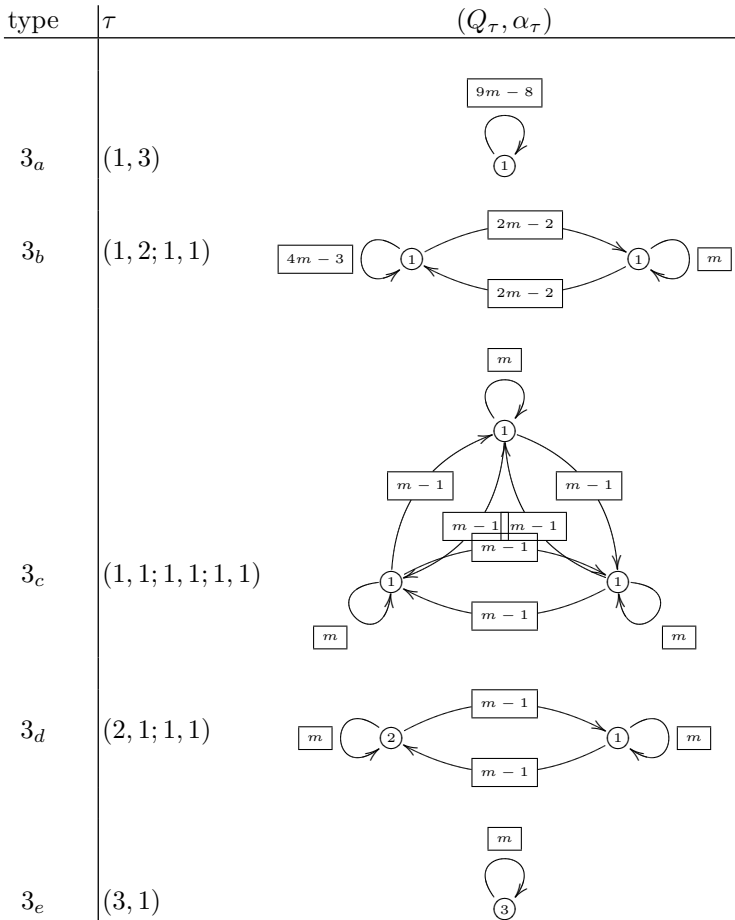
FIGURE 6.8: Local quiver settings for 3 \times 3 matrices.
