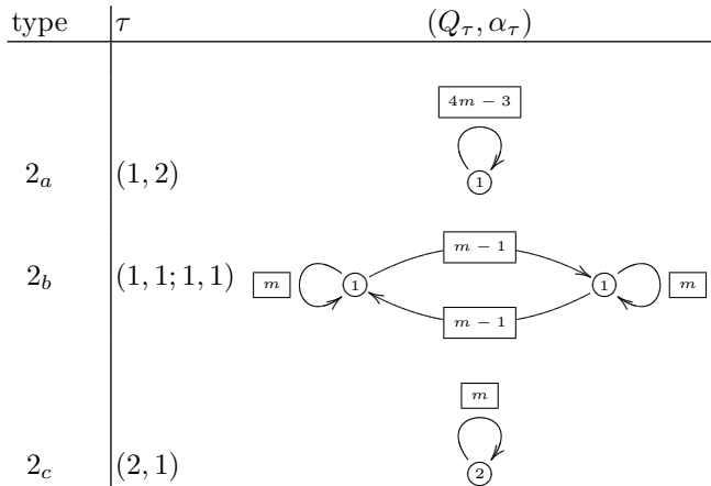
FIGURE 6.6: Local quiver settings for 2 \times 2 matrices.
