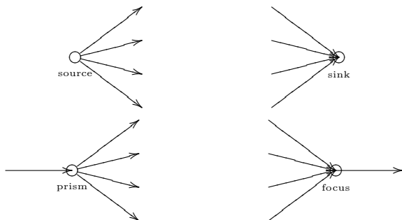
FIGURE 4.7: Vertex terminology.
