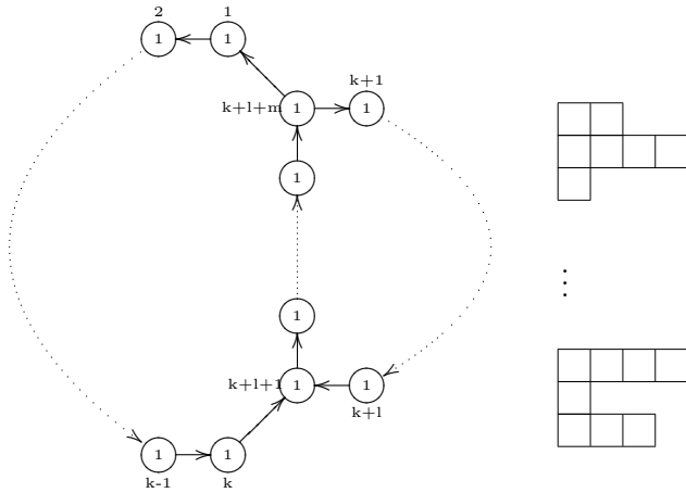
FIGURE 6.10: Local quiver settings for surface orders.
