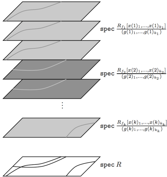
FIGURE I.3: An étale cover of X = \text{spec } R .
