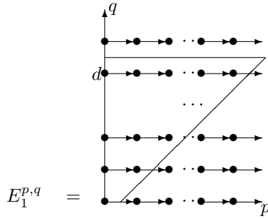
FIGURE 3.6: Coniveau spectral sequence.
