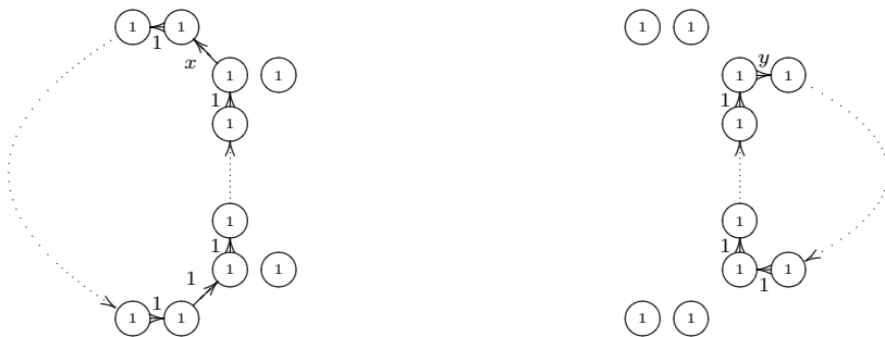
FIGURE 5.6: Proper semisimples of A_{klm} .
