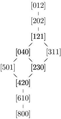
FIGURE 2.2: Orbit closures in \text{rep}_8 \mathbb{C}[x]/(x^3) .
